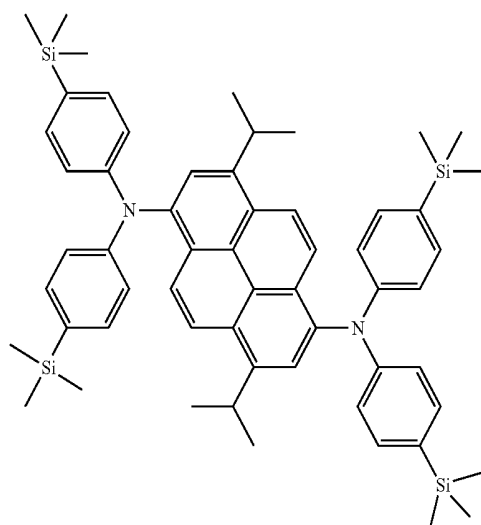
Compound C
