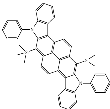
Compound D
