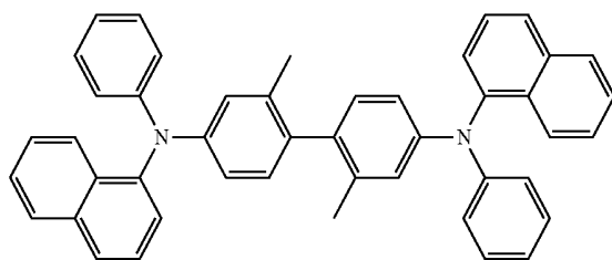
methyiated NPB
