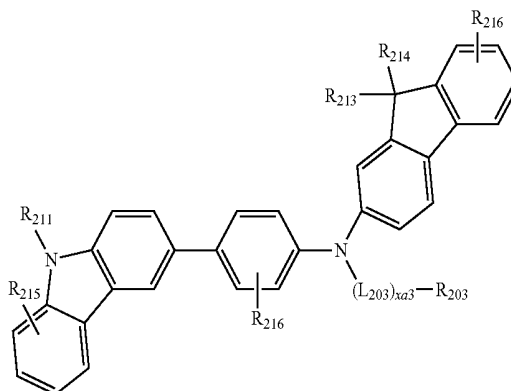
Formula 201A-1
