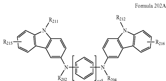
Formula 202A
