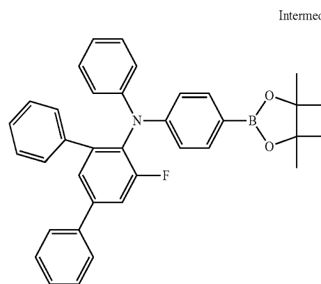
Intermediate I-13
