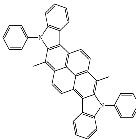
Compound E
